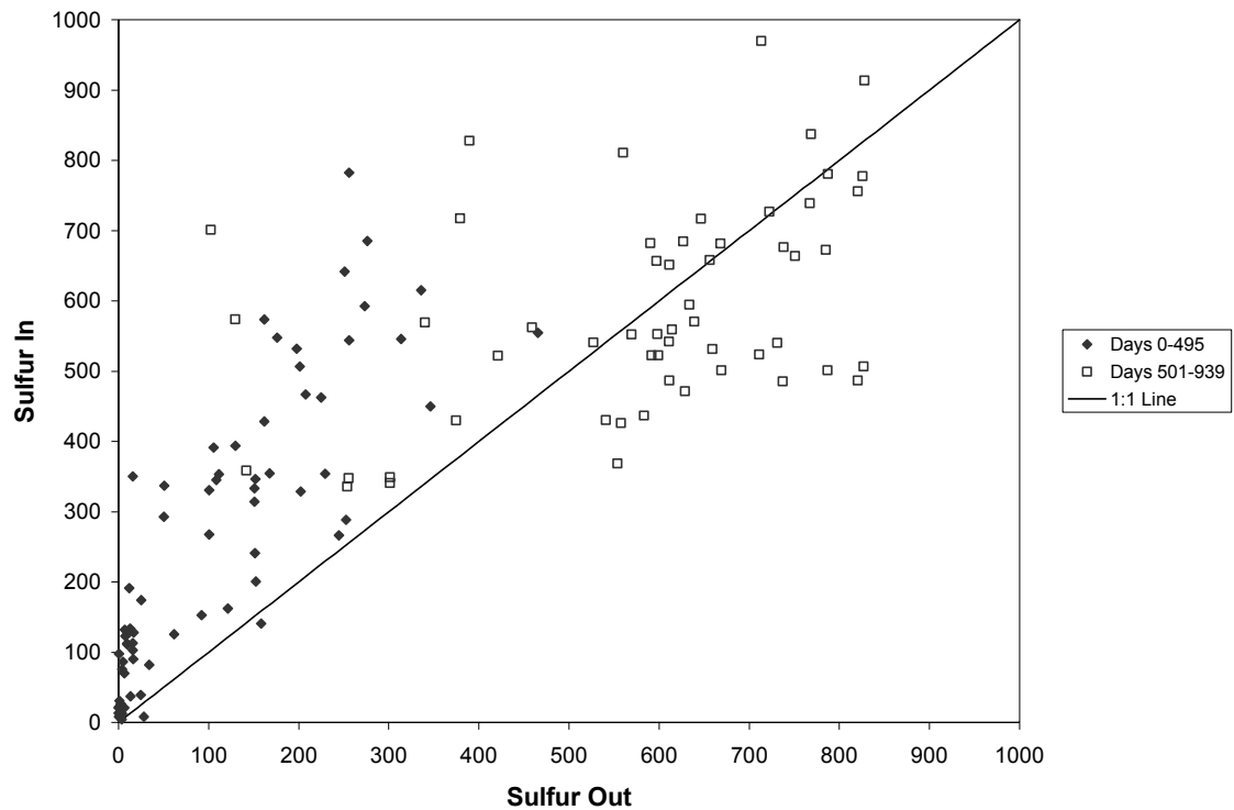
Figure 3-10 Sulfur mass balance for R3.
